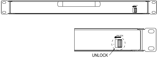
2-1.3 unlocking
