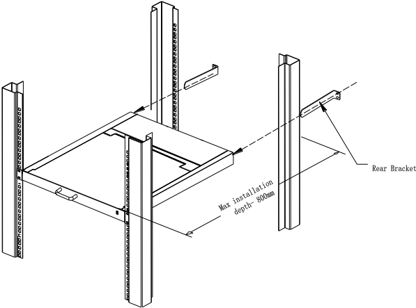
1-2.1 rack mounting (1)
