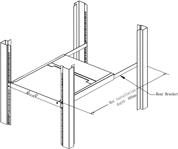
1-2.2 rack mounting (2)
