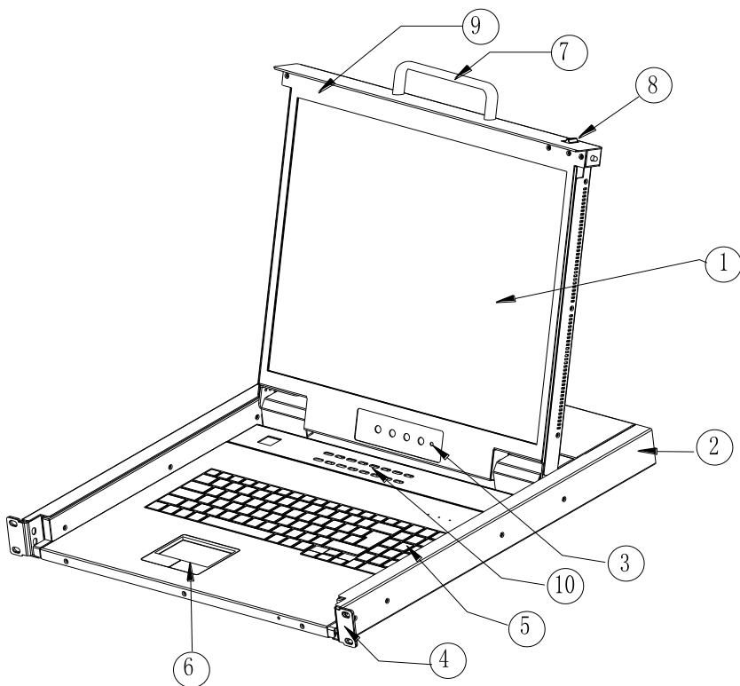
1-1.1 front view
